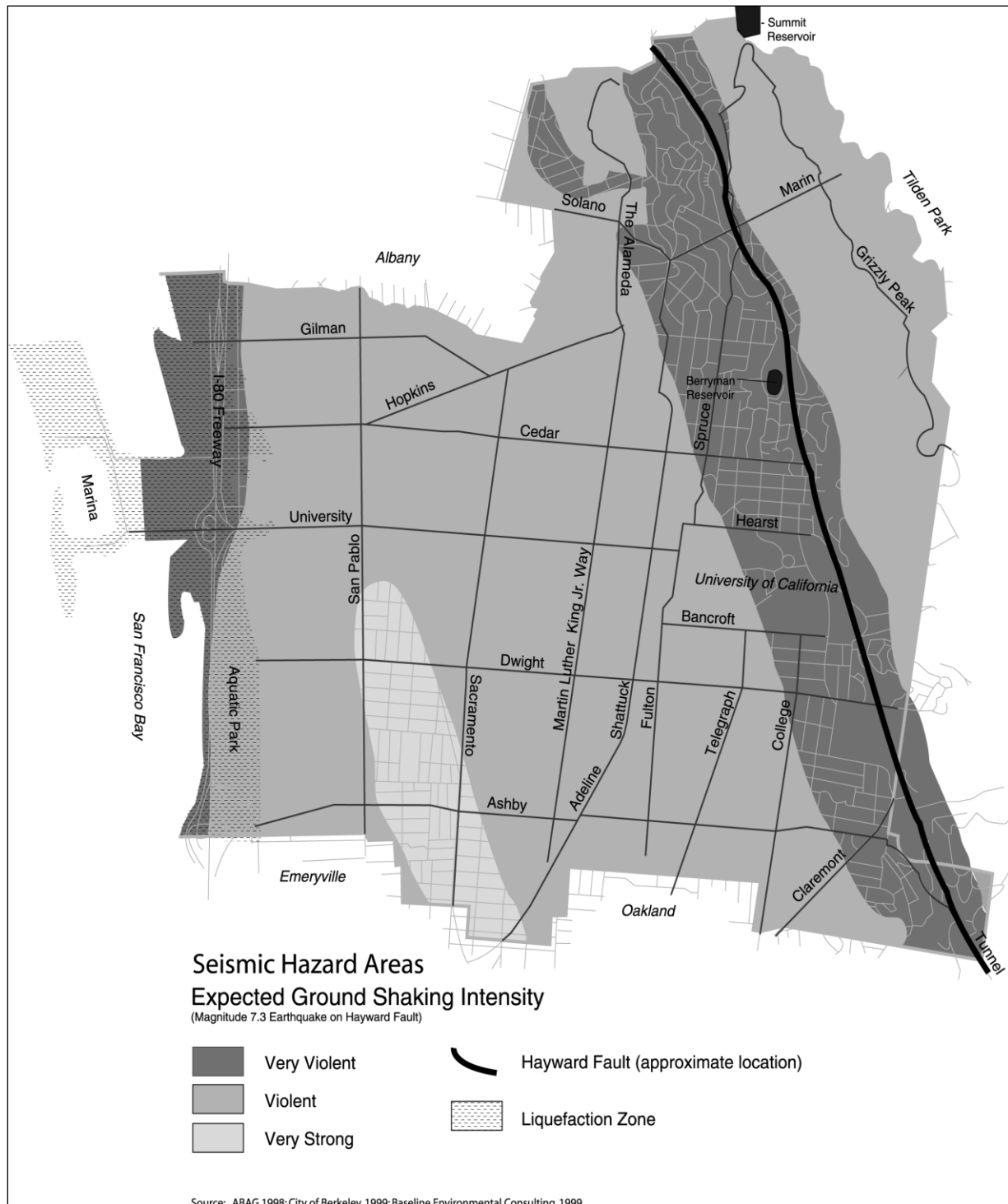
Figure 12 – Ground Shaking Intensity
