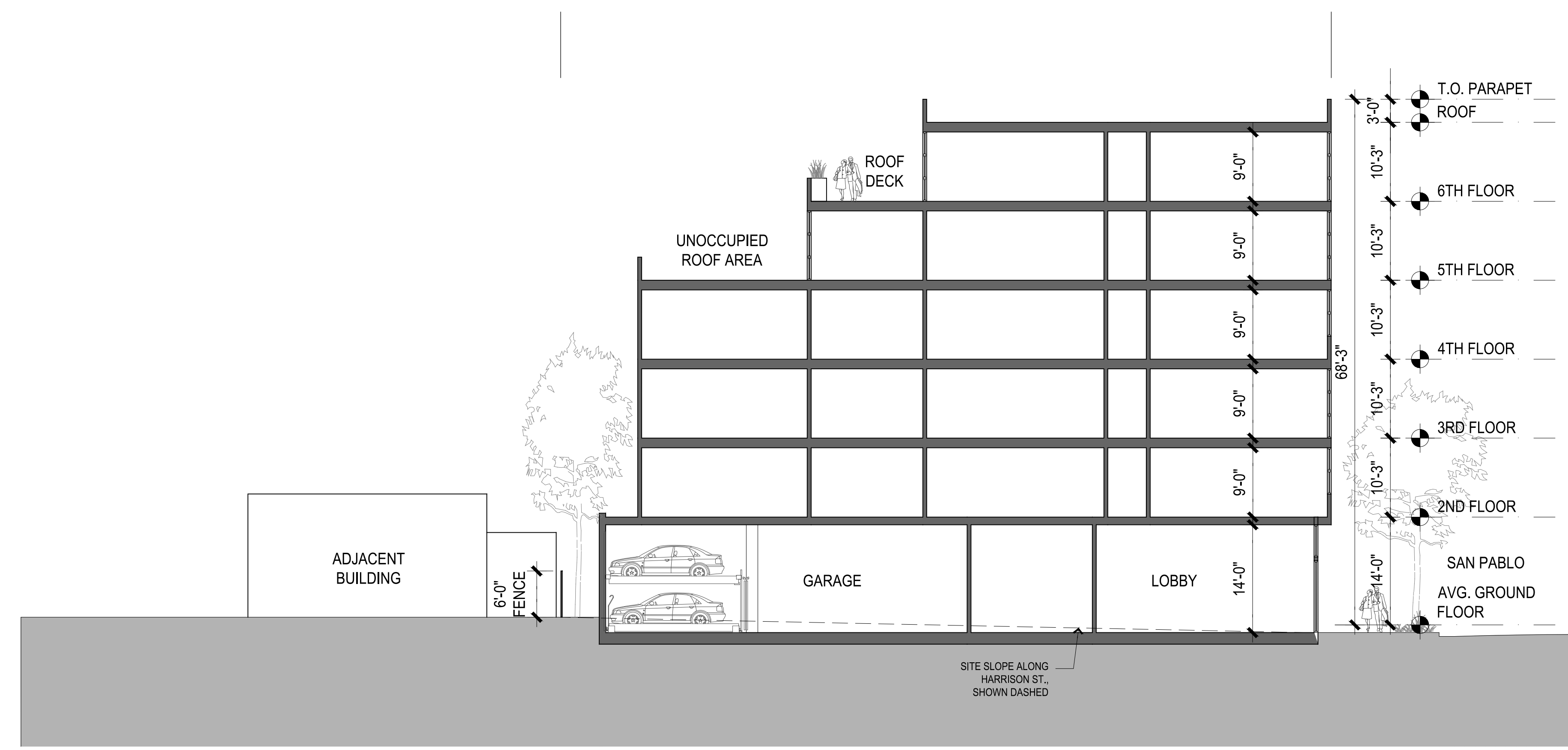
2 E-W SECTION THROUGH PODIUM GARDEN 3/64"=1'-0" @ 11X17 3/32"=1'-0" @ 24X36
