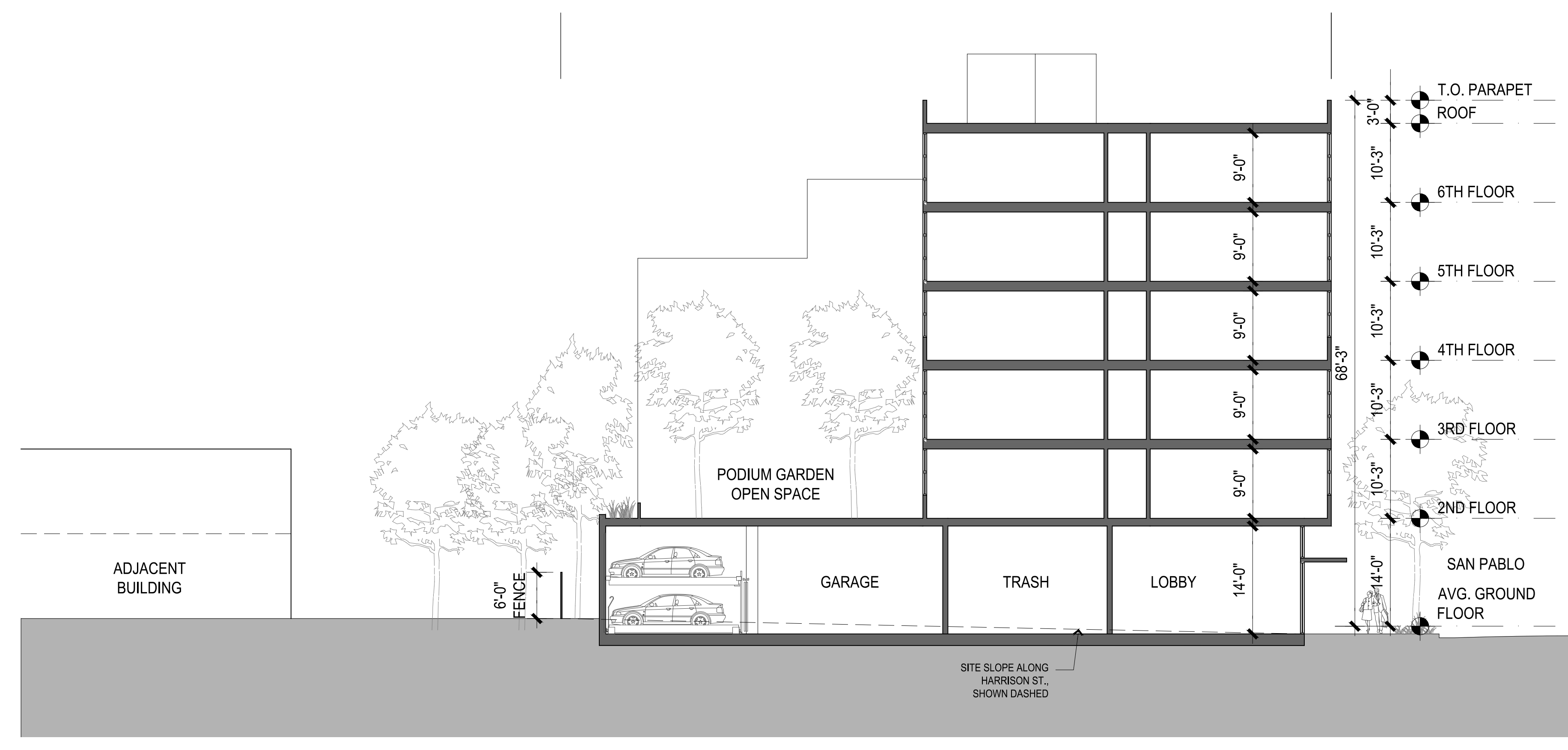
1 E-W SECTION 3/64"=1'-0" @ 11X17 3/32"=1'-0" @ 24X36
