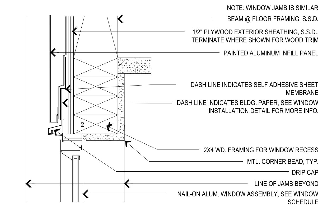
8 HEAD @ FILL PANEL 3"=1'-0"
