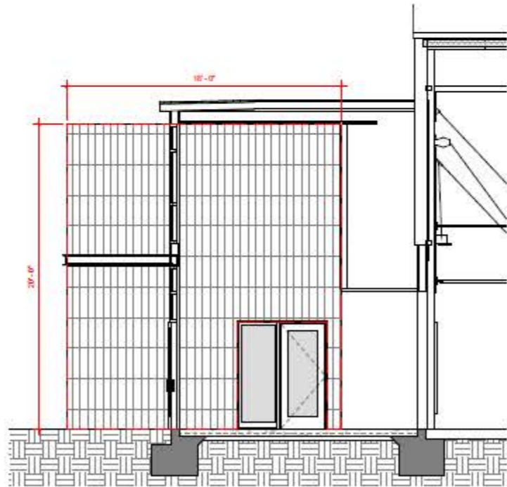
2 NORTH ELEVATION AND SECTION AT LOBBY 1/4" = 1'-0"
